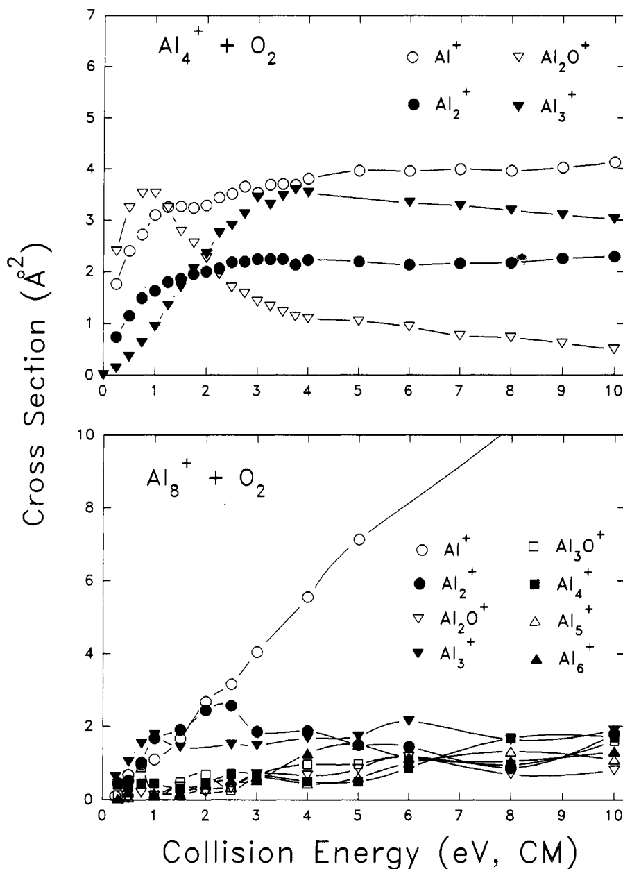
Figure 8. Absolute cross section for reaction of typical small aluminum cluster ions with O 2 . Note extensive fragmentation in the products, due to the large reaction exoergicity relative to the binding energy of Al x + .
