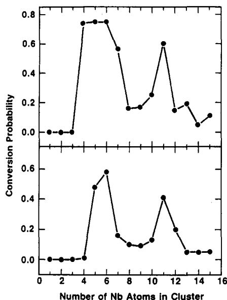
Figure 18. The probability for the reaction of \text{Nb}_x^+ (upper panel) and \text{Nb}_x (lower panel) with benzene to yield the completely dehydrogenated product \text{Nb}_x\text{C}_6^+ or \text{Nb}_x\text{C}_6 is plotted as a function of niobium cluster size. (Adapted and reprinted from ref 128. Copyright 1988 American Institute of Physics.)
