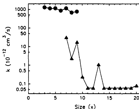
Figure 9. Rate constants k for the primary reaction of \text{C}_x^+ with \text{HCN} , plotted vs cluster size for the "linear" ( \bullet ) and "cyclic" ( \blacktriangle ) forms. The values for x = 11, 12 , and 14-20 are upper limits as no reaction was observed. The plot shows the existence of two isomers for x = 7-9 and the large drop in reactivity between x = 9 and 10 . (Data taken from ref 46.)
