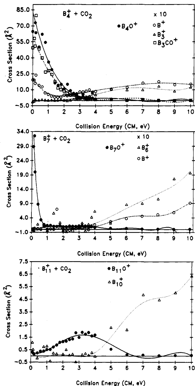
Figure 7. Absolute cross sections for reaction of several boron cluster ions with \text{CO}_2 . \text{B}_4^+ shows behavior typical of small boron cluster ions, \text{B}_{11}^+ is typical of clusters in the 8–14-atom range, and \text{B}_7^+ shows transitional behavior.
